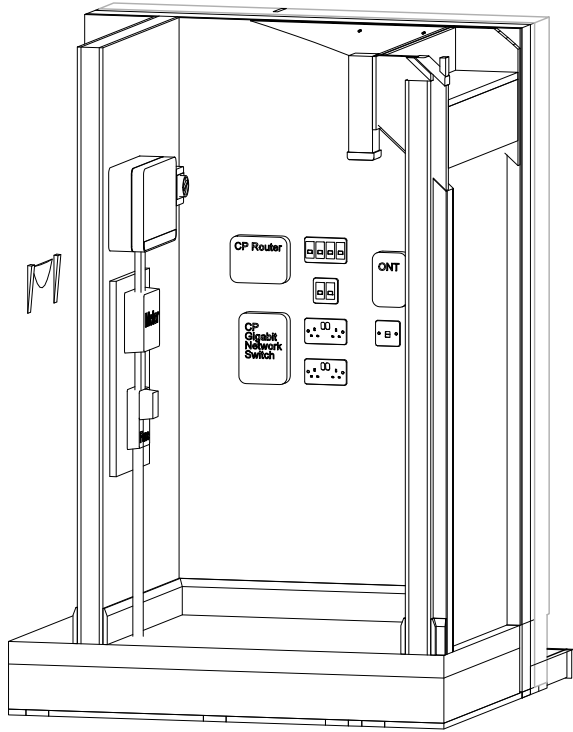
Plot 42 Internal cupboard layout 2 Mid Terrace Cup'd (View A)
